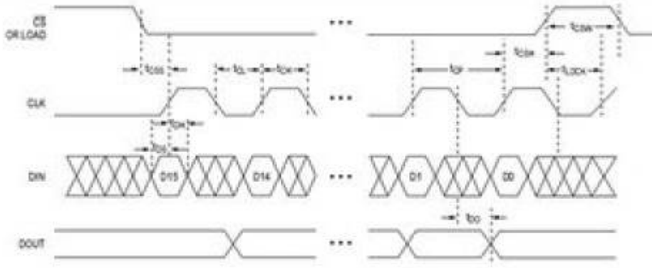
Figure 1. Timing Diagram
