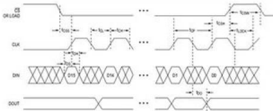
Figure 1. Timing Diagram
