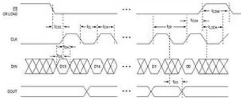
Figure 1. Timing Diagram
