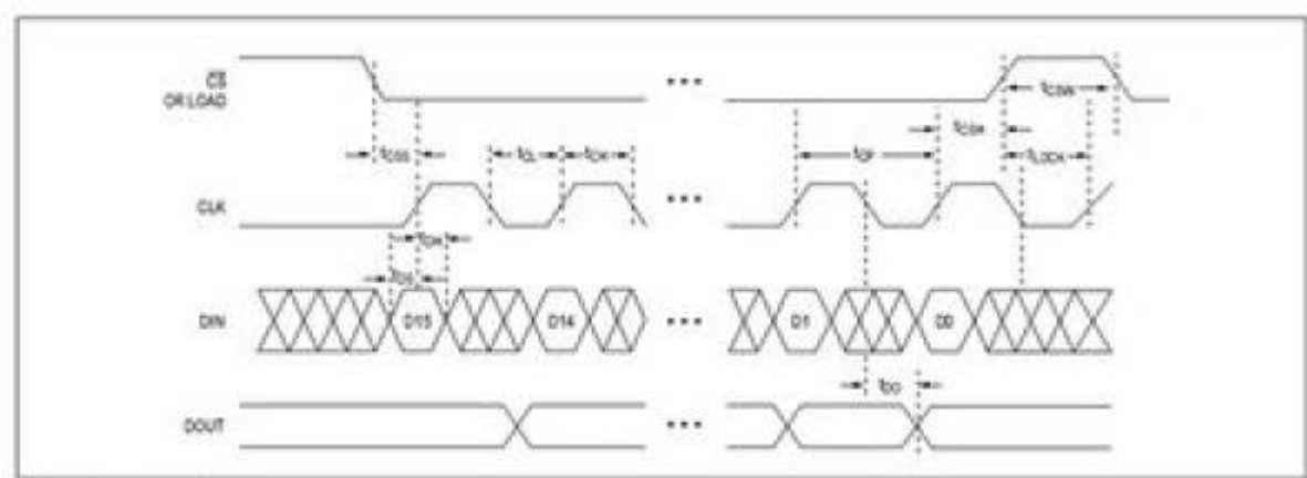
Figure 1. Timing Diagram
